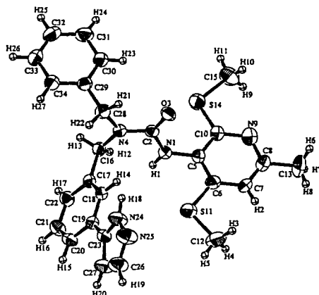
Figure 1. ORTEP drawing of FR186054 (2c) with crystallographic numbering scheme.
